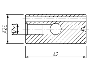
S17/D32AG3S6 pattino D32AG3S6
