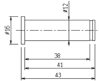
S17/030P perno / pin
