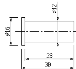
S17/031P perno / pin
