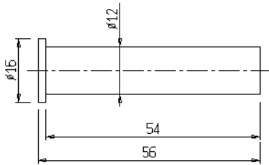
S17/030PL Perno da forare in macchina / pin to be drilled once fitted 3.81.78.03.0
