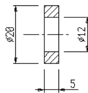
S17/032R rullino / roller 3.51.51.38.0
