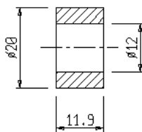
S17/031R rullino / roller WT32.33
