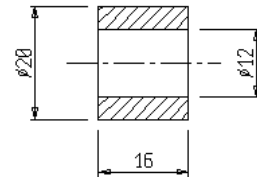
S17/030R rullino / roller 3.84.14.20.0 WT32.34
