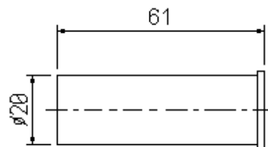
S8/031P Perno / Pin WT36.6
