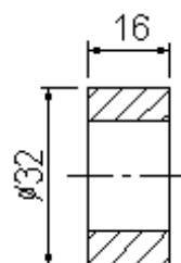
S8/031R Rullo / Roller WT32.8
