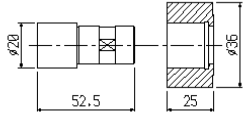
S5/031P (523) perno / pin
