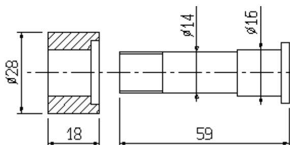
S5/032R (90) rullo / roller
