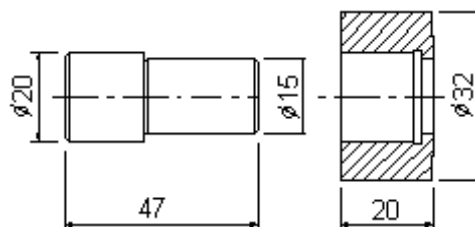
S4/031P perno / pin
