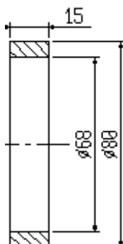
S4/008B anello / ring 383
