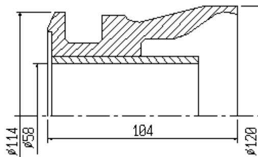
S4/001B campana / sleeve SD25 376+329
