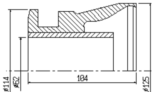
S4/001 campana / sleeve SD32 376+329
