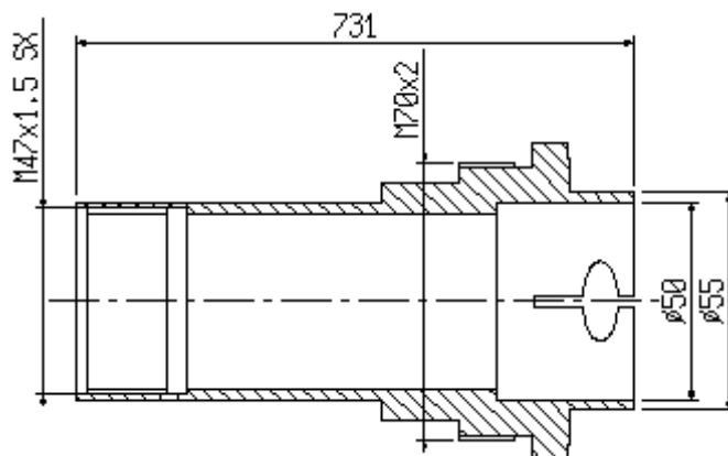
S4/010 tubo portapinza / collet tube 341
