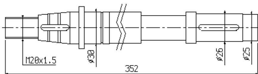
S4/058 albero / shaft SD63d121a
