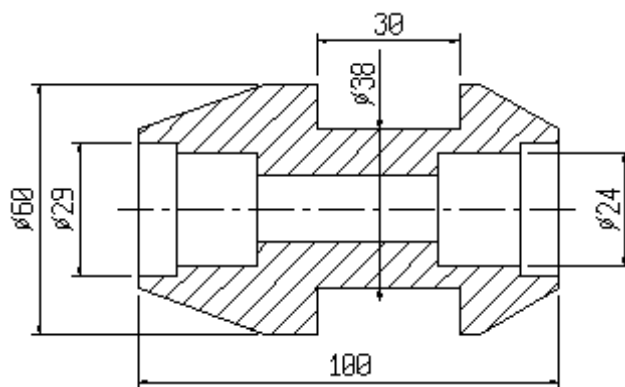
G9/050B rullo / roller
