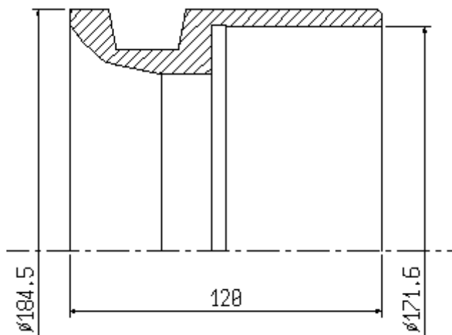
G9/001 campana/sleeve AS82
