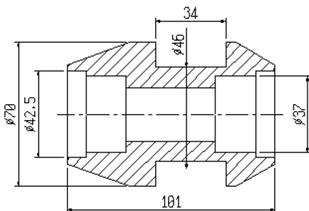
G9/050A rullo / roller
