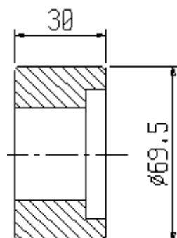
G9/035R rullo / roller
