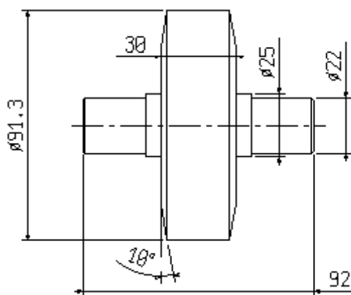
G5/040B rullo / roller
