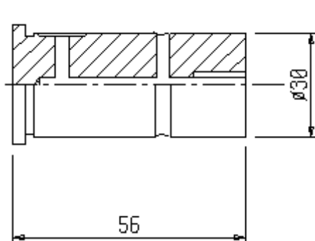
G9/030P perno / pin 305-08-1410
