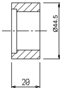
G9/030R rullo / roller 305-08-1420
