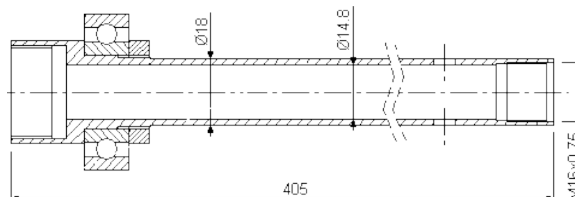
R1/012E (AS12/10-6) Feed tube for 85mm stroke Tube d'avance, ravitaillement 85mm
