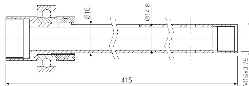
R1/012 (AS12/10-4) Phaseable Feed tube - with slot Tube d'avance orientable
